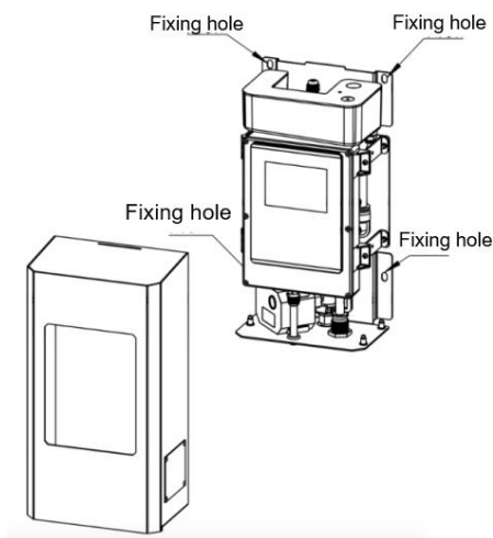
Fig.5 Fixing hole
