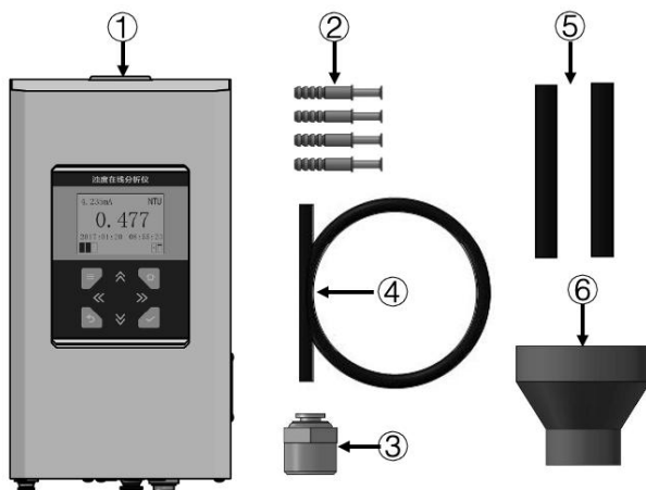
Fig.3 Installation components
