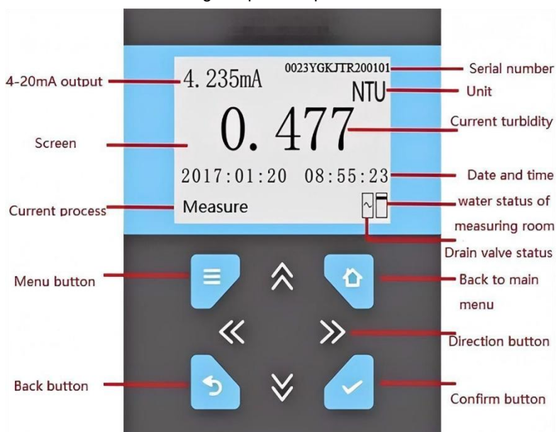
Fig.8 Operation panel
