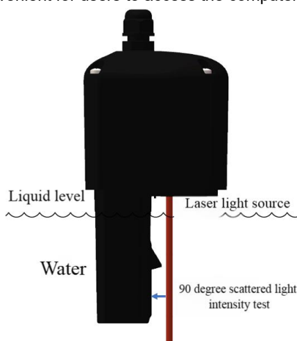
Fig.1 Measurement principle
