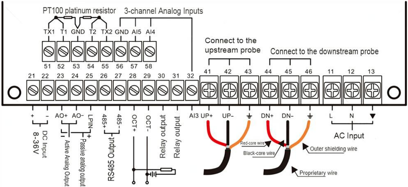
Fig.1 Wall-Mounted Host Terminal Block
