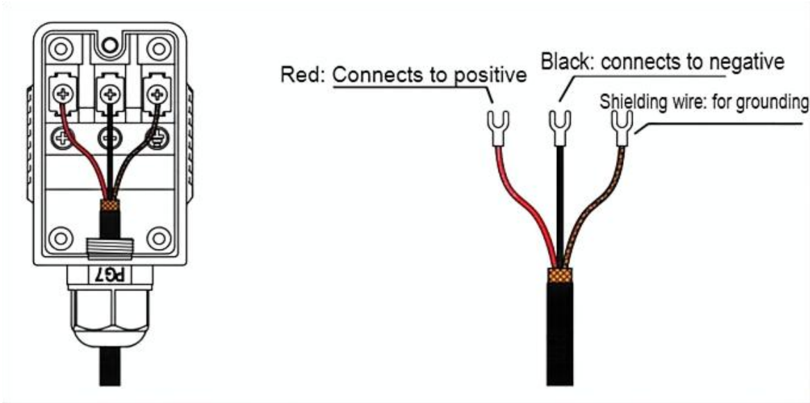
Fig.3 Wiring Diagram Of Clamp-On Sensor
