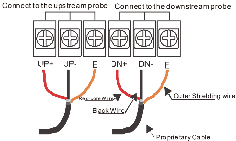
Fig.6 Sensor Connecting To The Host
