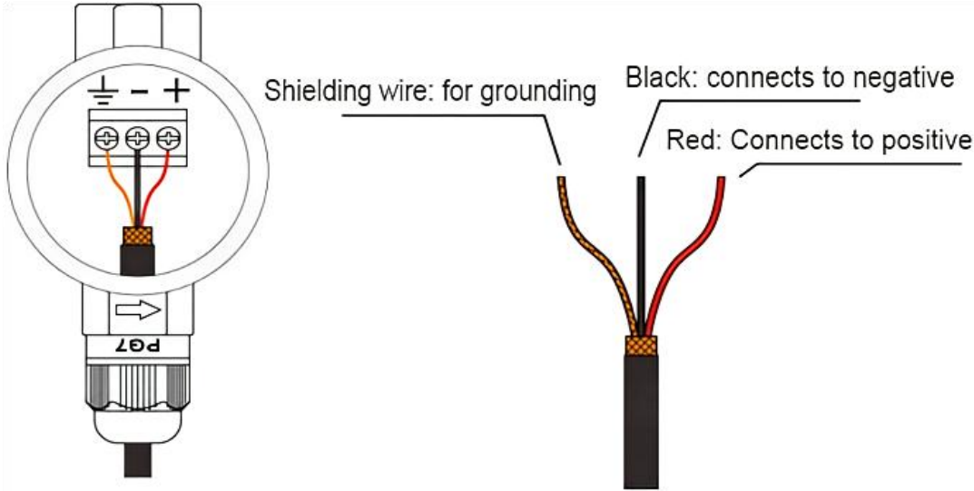
Fig.4 Wiring Diagram Of Insertion Sensor
