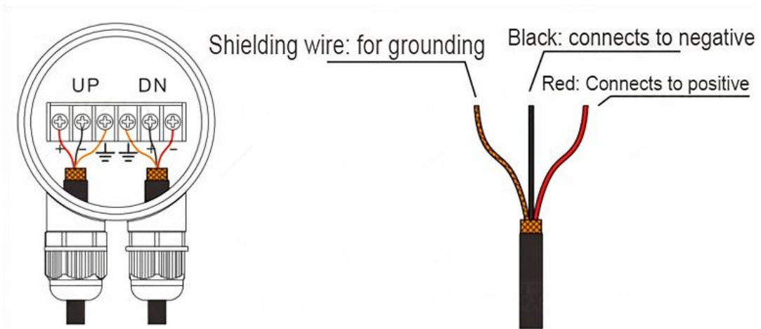
Fig.5 Wiring Diagram Of The Remote Inline Sensor
