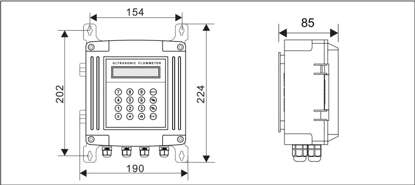
Wall mounted type dimension
