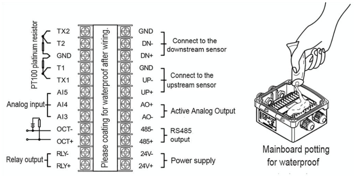
Fig.2 Integrated Host Terminal Block
