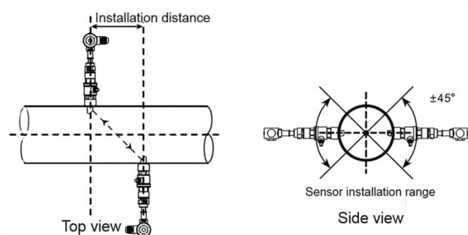
Fig.16 Z method installation diagram
