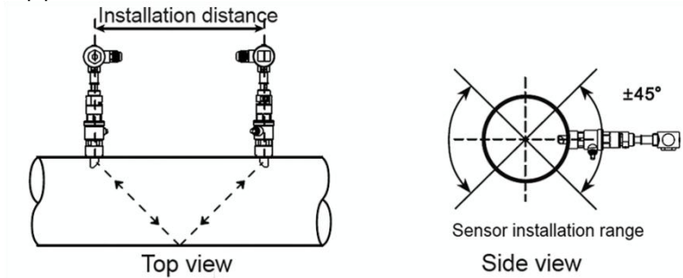
Fig.15 V method installation diagram
