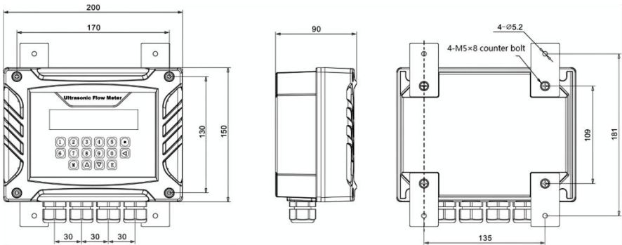
Fig.3 Main unit dimensions (unit: mm)
