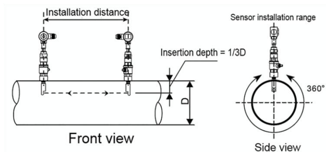
Fig.17 Parallel Insertion
