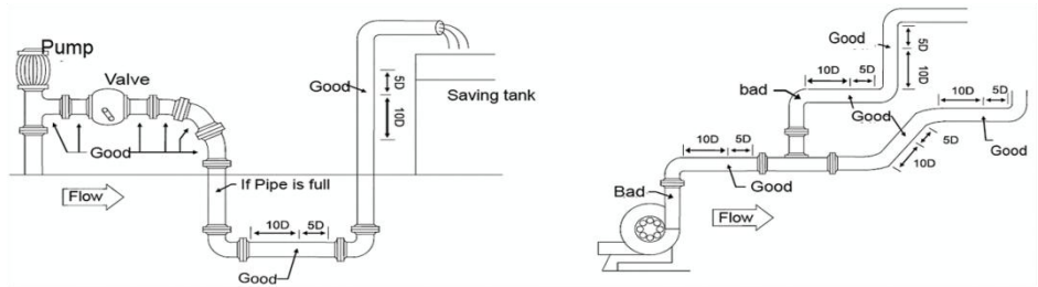
Fig.8 Installation sites for stable flow
