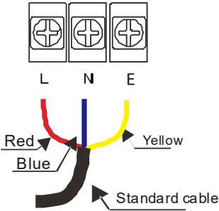
Fig.26 220VAC Power Supply Connection
