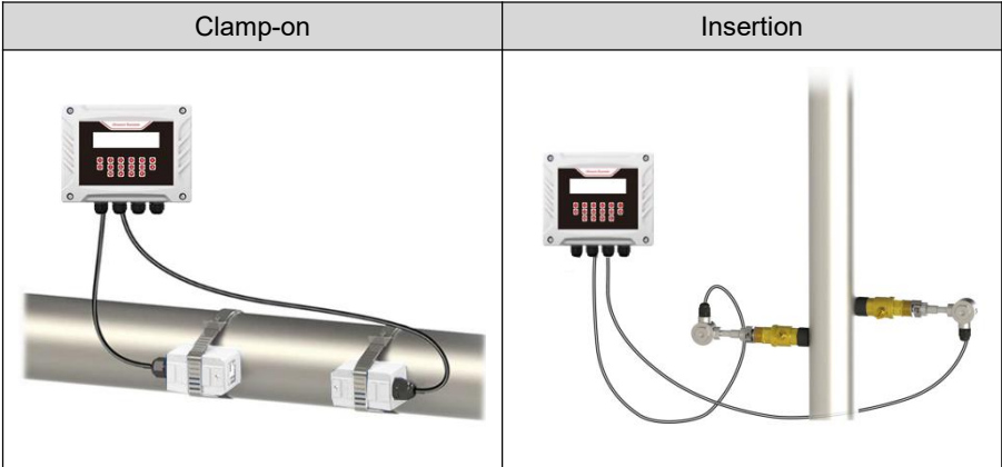
Fig.2 Measuring system
