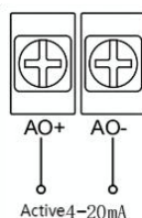
Fig.28 Analog Output Wiring
