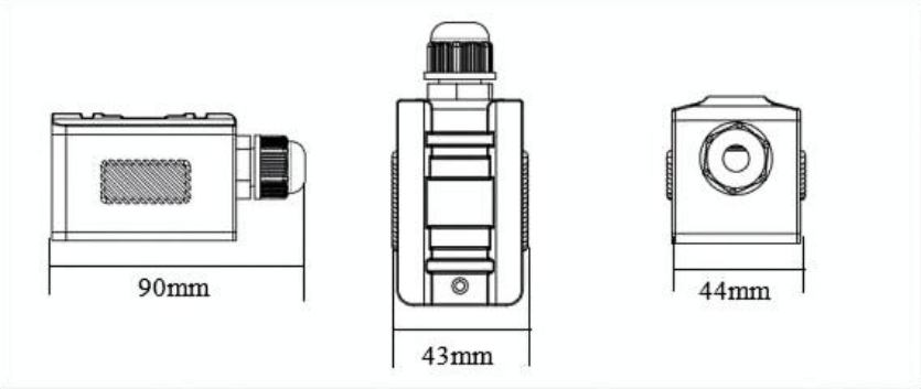
Fig.4 Dimensions
