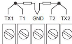
Fig.30 Heat Measurement Wiring
