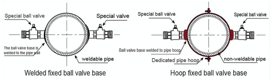
Fig.20 Fixing ball valve base
