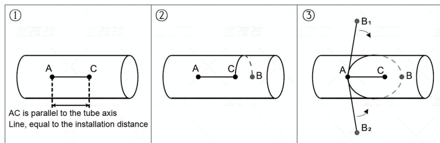
Fig.19 Z method installation location
