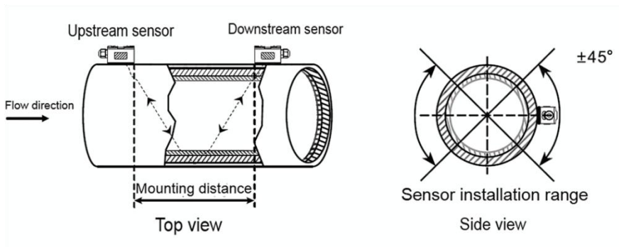
Fig.9 V-method installation
