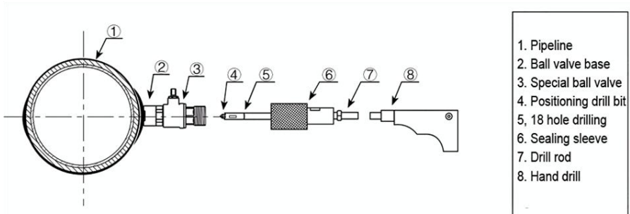
Fig.21 Drilling
