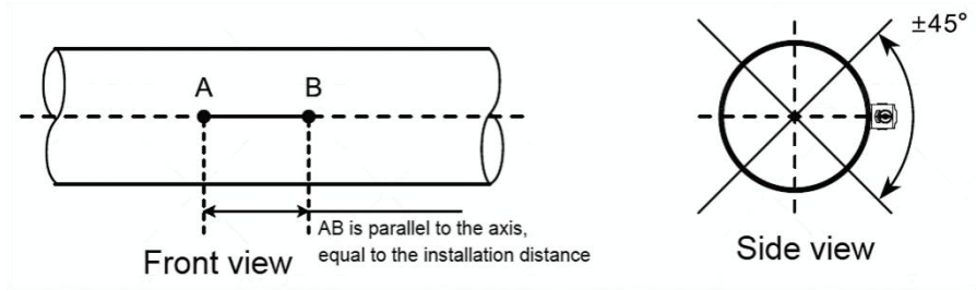
Fig.11 V-method installation site determination
