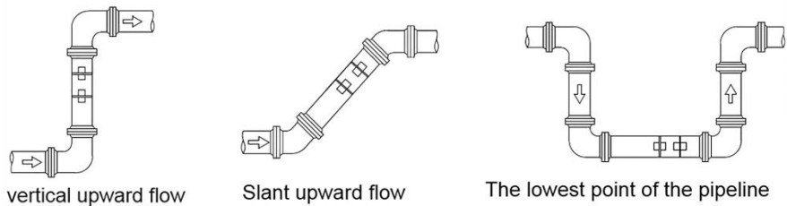
Fig.7 Full pipe installation site
