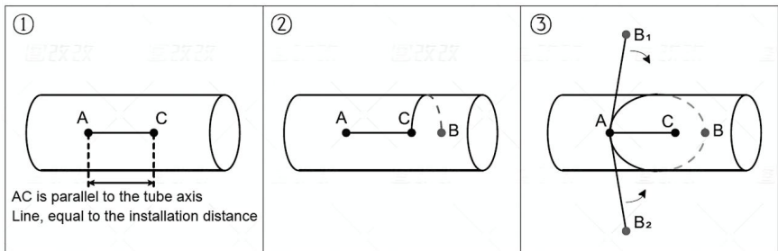
Fig.12 The Z-method site determination
