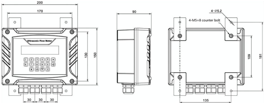
Fig.6 Main unit installation (unit: mm)
