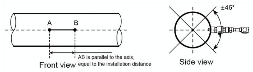
Fig.18 V method installation location
