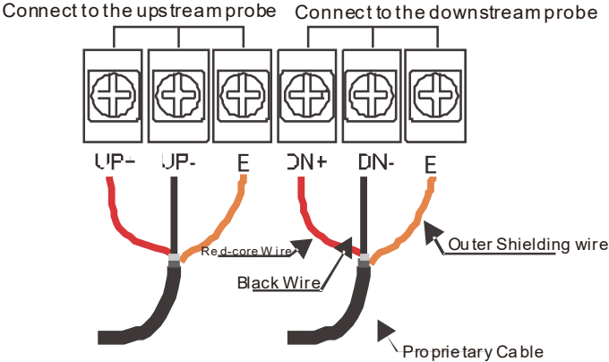
Fig.24 Sensor connecting to the host
