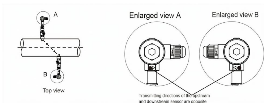
Fig.22 Adjusting transmitting direction
