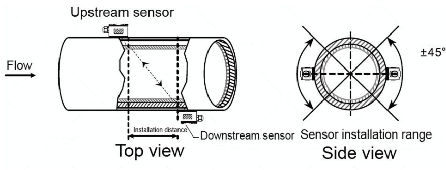
Fig.10 Z-method installation
