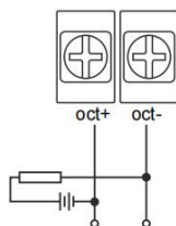
Fig.27 Pulse/frequency output wiring
