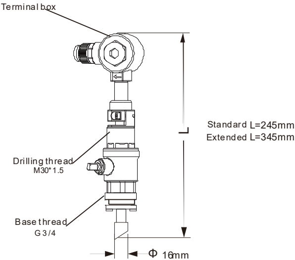
Fig.5 Dimensions
