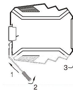
Fig.3 Disassembly method
