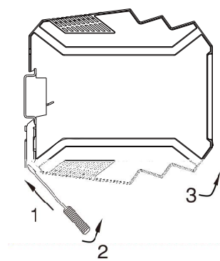
Fig.2 Disassembly method
