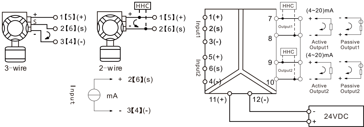
Wiring diagram of Double-channel input and Double-channel output:dx
